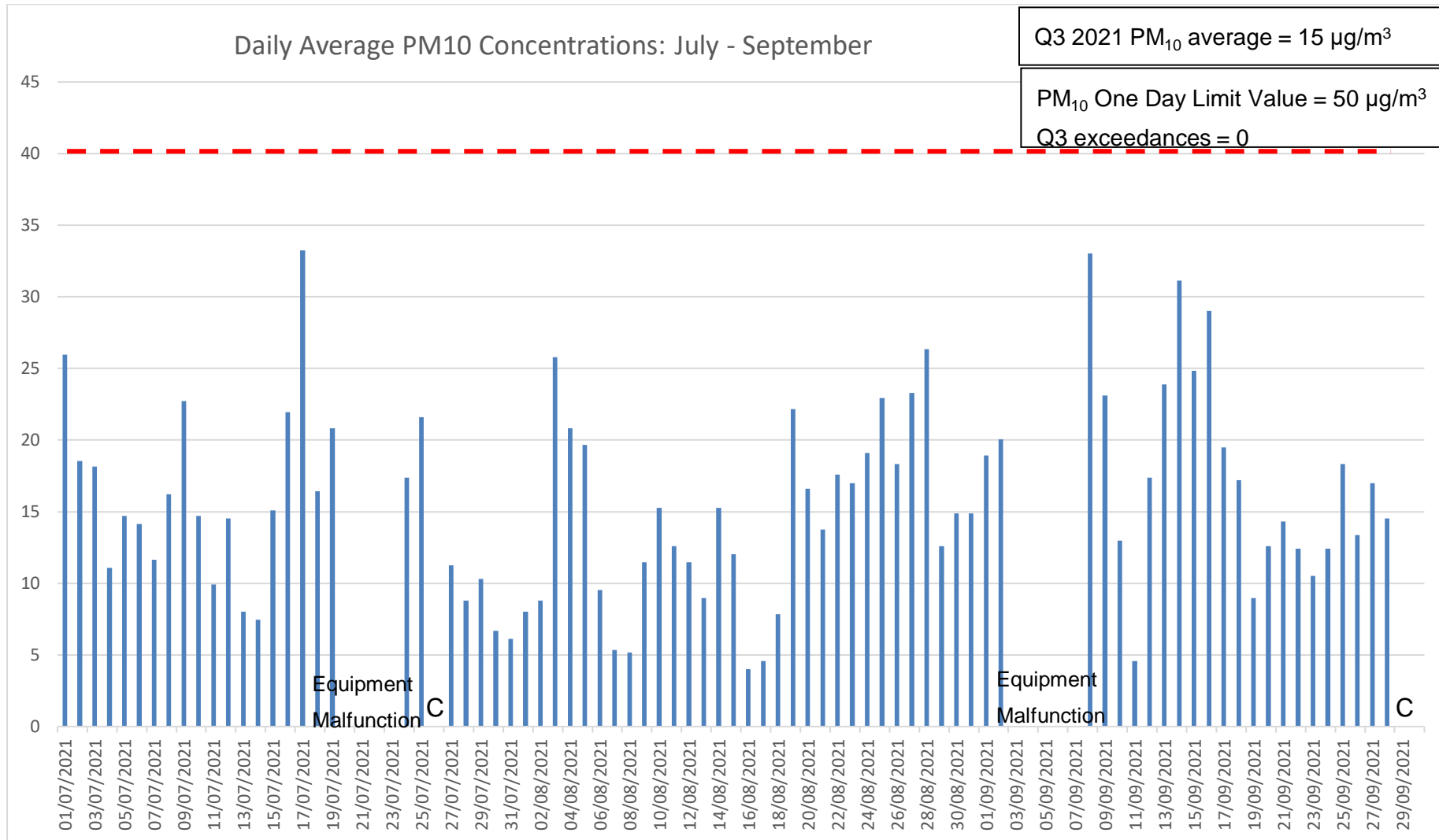
Figure 5 Daily Average PM 10 Q3 2021
