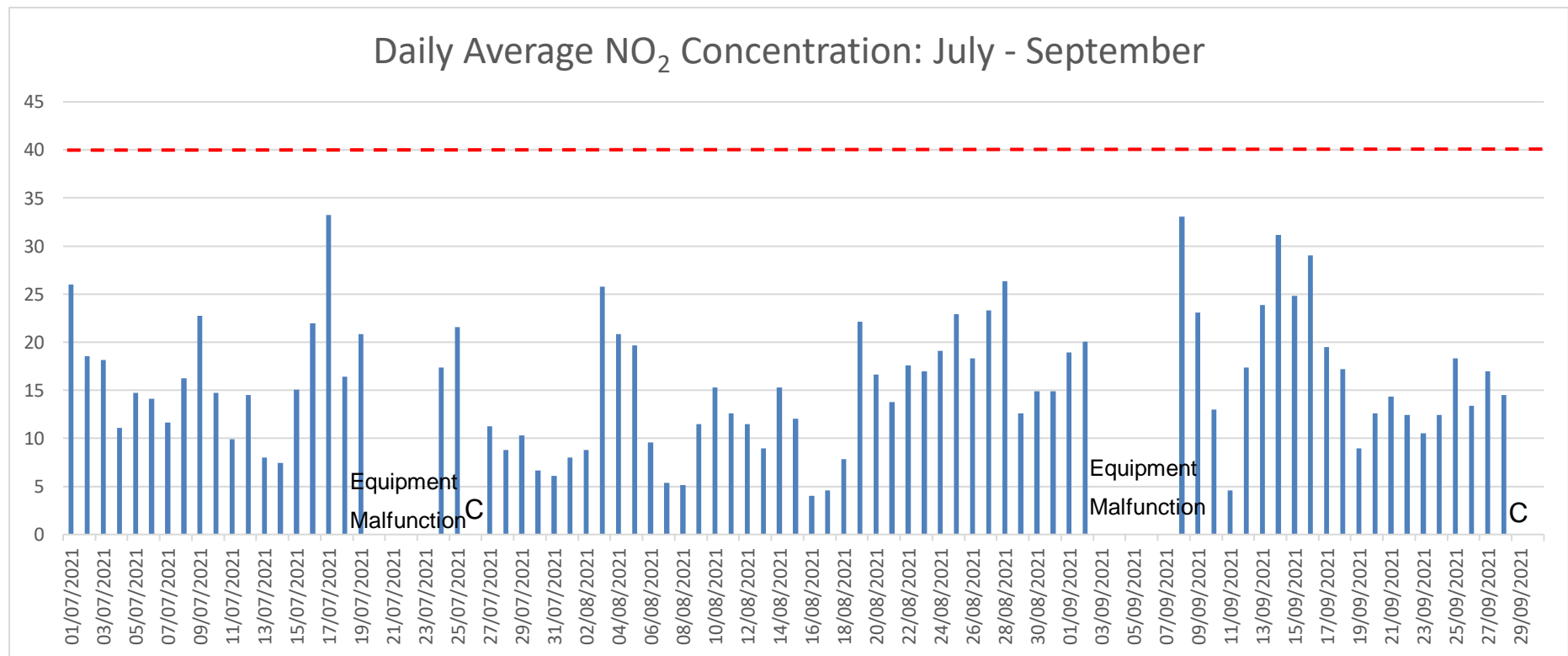
Figure 4 Daily Average NO 2 Q3 2021
