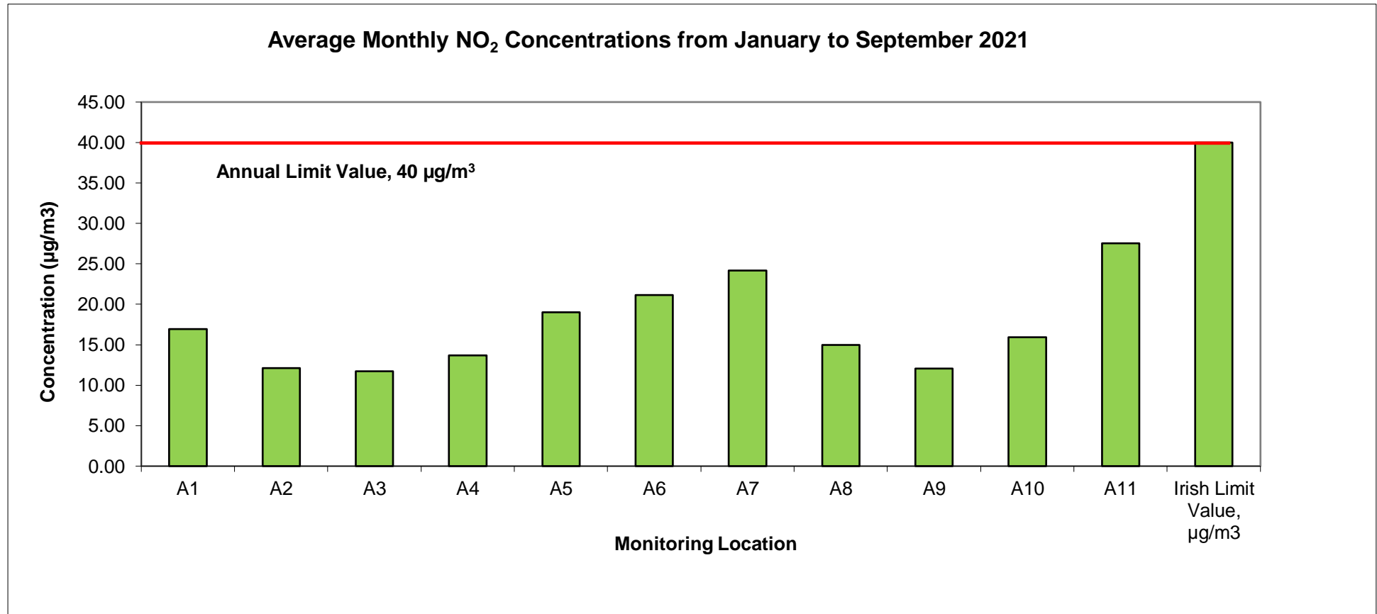
Figure 2 Average Monthly NO 2 Concentrations Q3 2021
