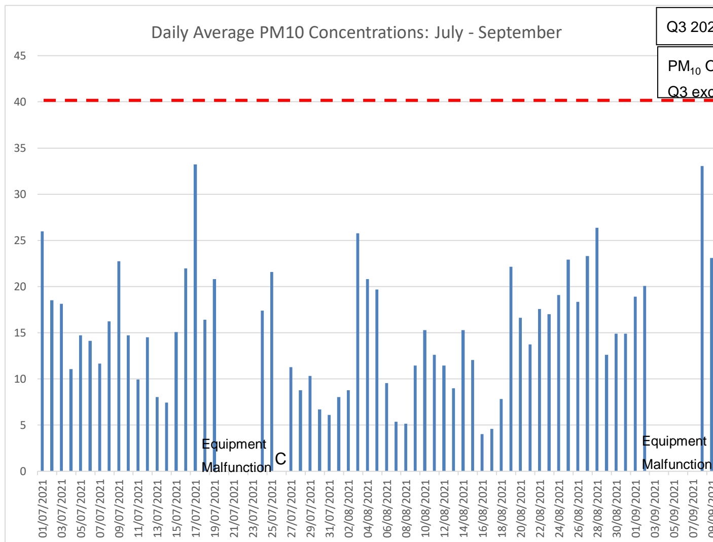
Figure 5. The average PM 10 was calculated as 13 µg/m 3 . The Regulations set a 24-hour PM 10 limit value of 50 µg/m 3 , and an annual mean limit value of 40 µg/m 3 as shown in Table 2.
